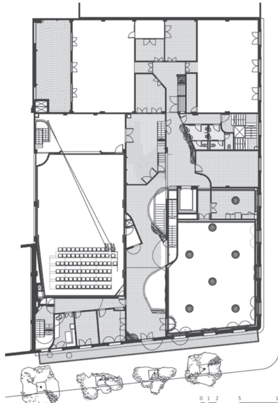
Plan etaj 1 / First Floor Plan
